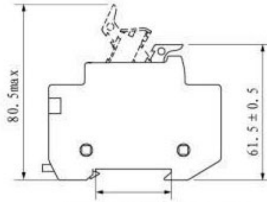
Equipped with TH35-7.5 mounting rail
